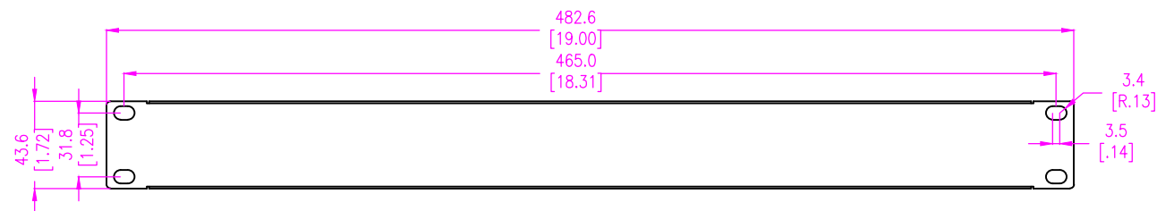
FRONT VIEW
